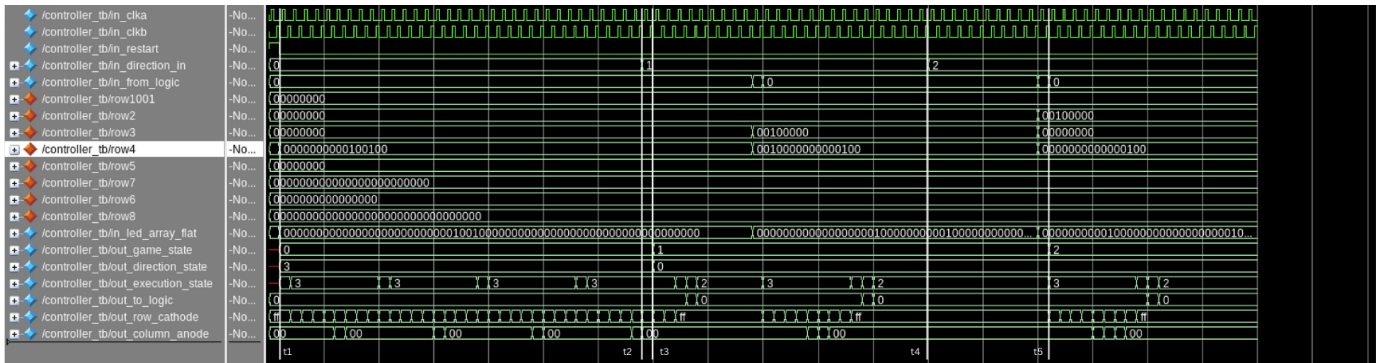
Fig. 3. Pre-synthesis Questa simulation of Controller module.
