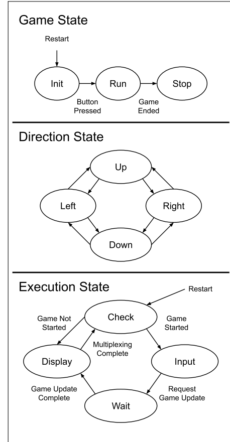
Fig. 1. State transition diagrams of each FSM in the Controller Module.
