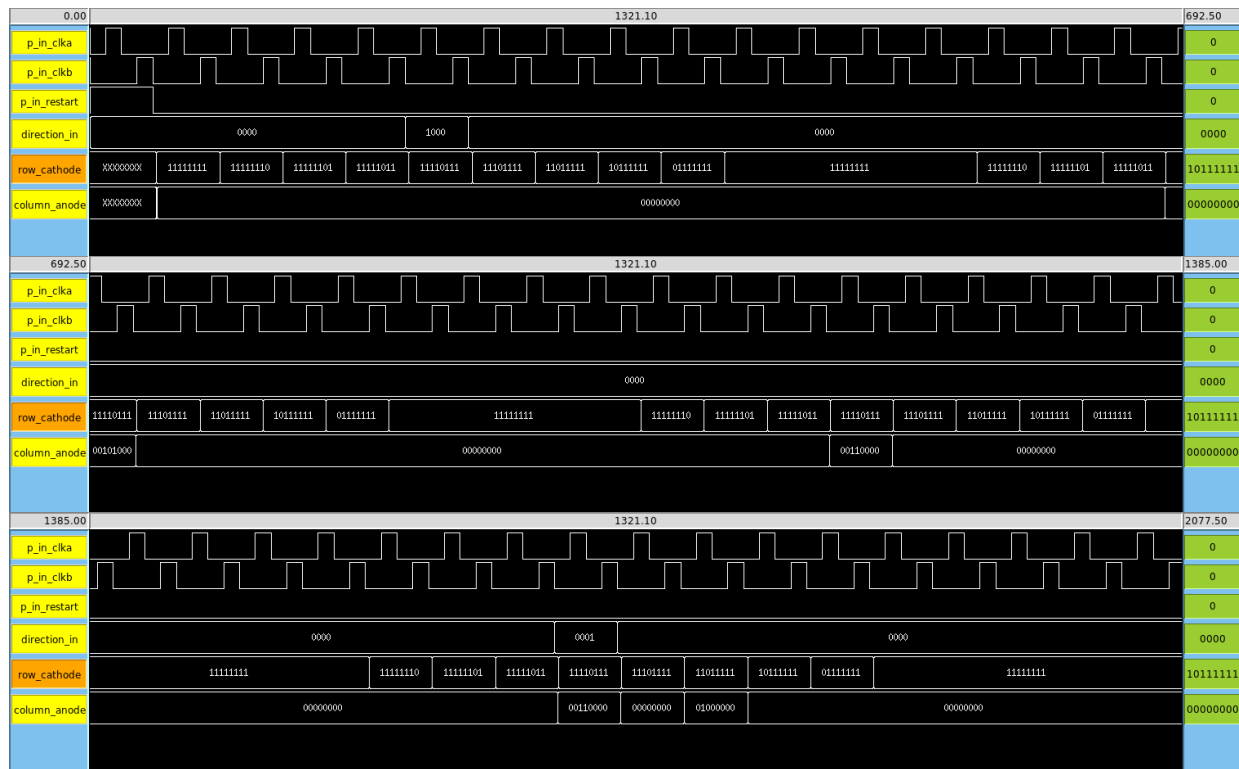
Fig. 22. IRSIM simulation of the design, from the padframe.
