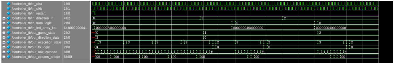
Fig. 19. Post-synthesis Questa simulation of Controller module.
