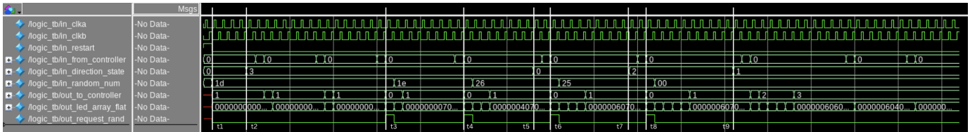
Fig. 4. Pre-synthesis Questa simulation of Logic module.
