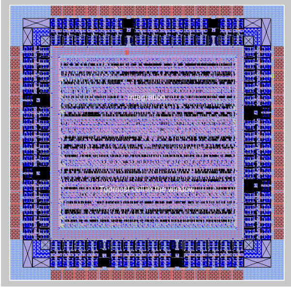
Fig. 16. Fully integrated core with padframe.
