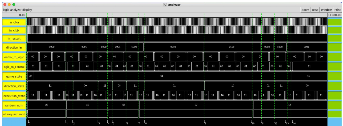
Fig. 12. IRSIM simulation of the core design.
