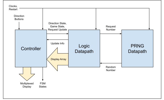
Fig. 2. Block diagram of top module.
