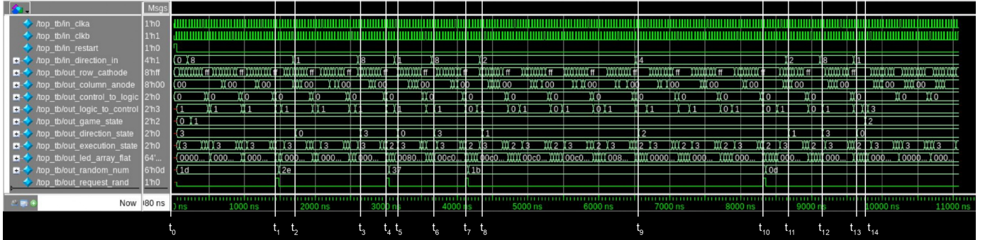
Fig. 6. Pre-synthesis Questa simulation of Top module.
