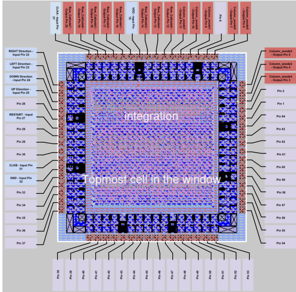
Fig. 17. 64-Pin PadFrame with pinmap (unused pins are configured as inputs).
