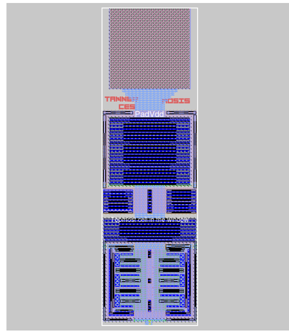
Fig. 15. Vdd pad provided by OSU.
