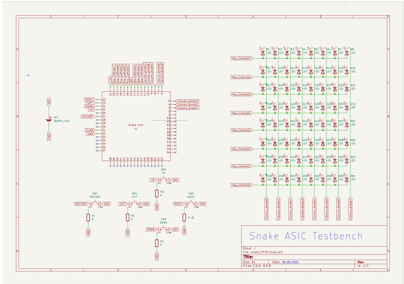
Fig. 24. Schematic of circuit required to test Snake ASIC.
